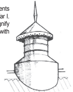
Woodworkers' Roof Ventilator Small - Height 980mm min. diameter - 200mm Base diameter 360mm Large - Height 1200mm min. diameter - 280mm Base diameter 500mm RE1
