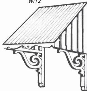
Woodworkers' Sweep Skillion Shown with fretwork fascia option Overhang 565 mm Height 1300 mm WH 4
