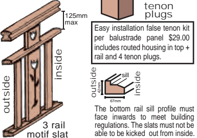
TB10 - 3 RAIL SLAT BALUSTRADE showing double motif center panel
